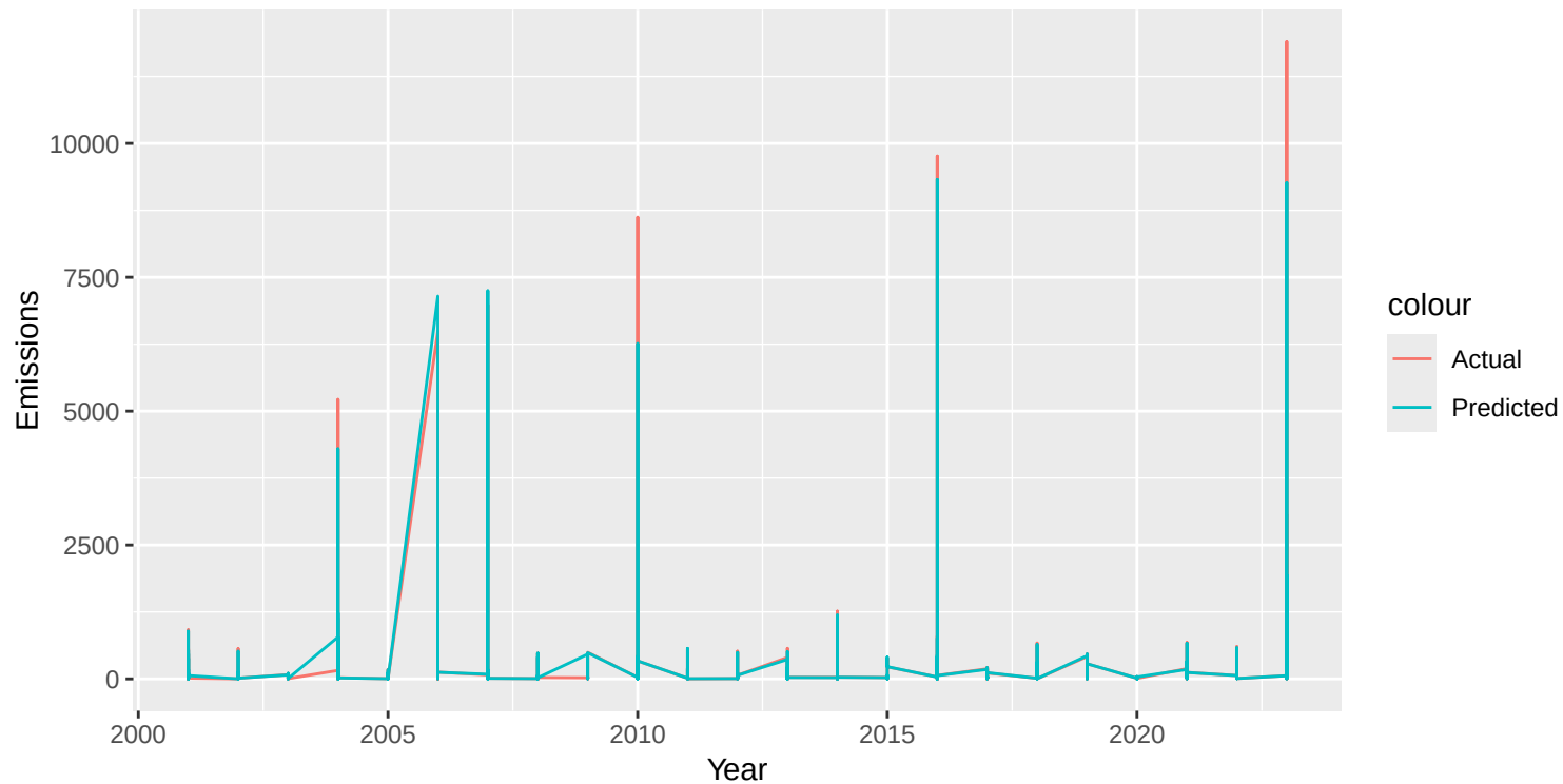
Actual vs Predicted Emissions by Year (Random Forest)
